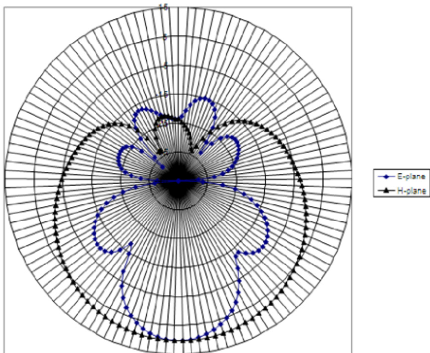
Antenna Field Pattern
