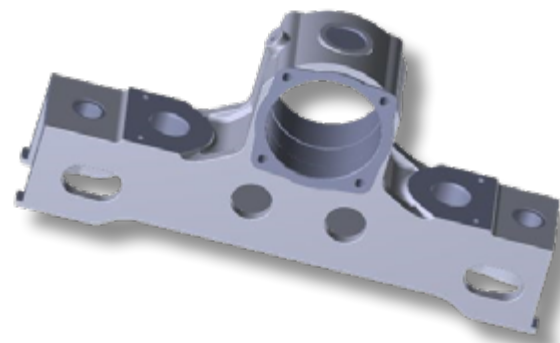
PRD16185637 Light Rail Vehicle Journal Box
