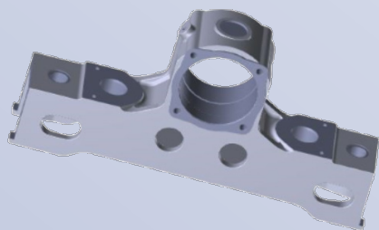
Obsolete CAF Timken cast/machined axle box manufactured in-house by PowerRail
