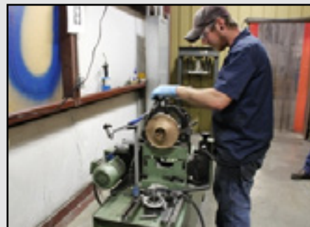
Balancing Impeller
