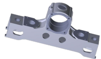
Obsolete CAF Timken Journal Box manufactured in-house by PowerRail
