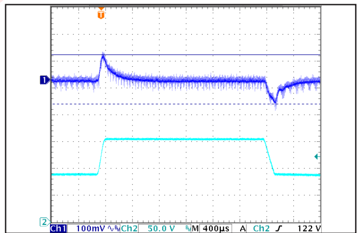
Figure 6: Output voltage response to step-change in input voltage (1V/ \mu s ). Load cap: 1 \mu F ceramic and 15 \mu F tantalum capacitors. Ch 1: V_{out} , Ch 2: V_{in} .
