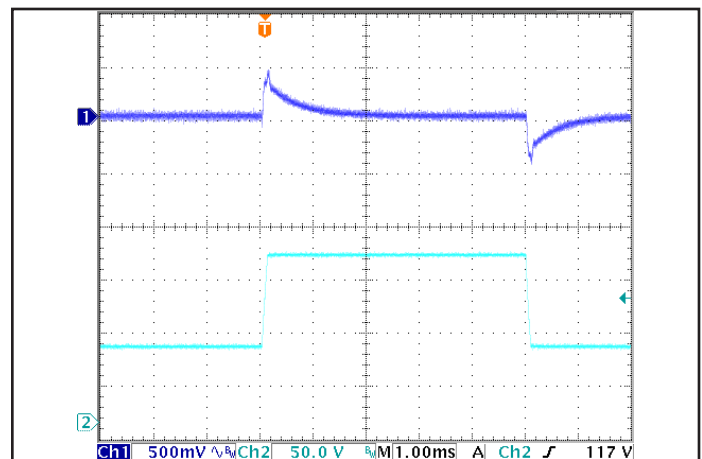
Figure 6: Output voltage response to step-change in input voltage (650V/ms), at Max. load current. Load cap: 15μF tantalum cap and 1μF ceramic cap. Ch 1: Vout, Ch 2: Vin.
