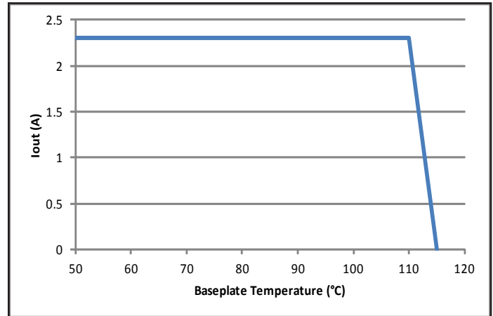
Figure 4: Maximum load current vs. baseplate temperature when conductively cooled. Note: The system design must provide a suitable thermal path that maintains the baseplate temperature below 110 °C.
