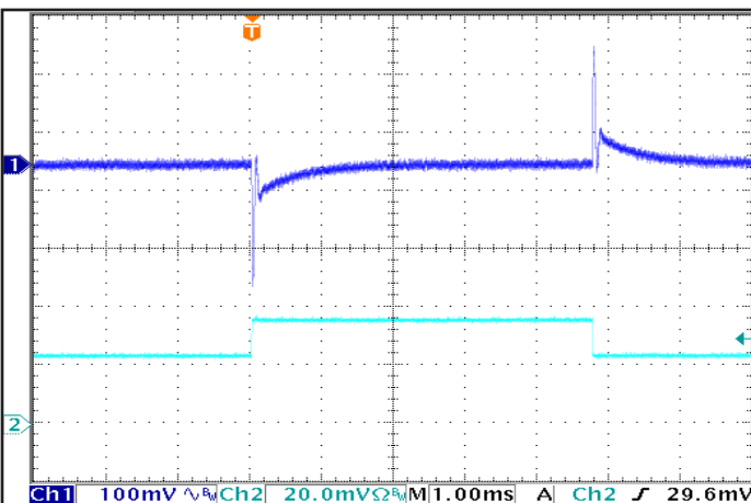
Figure 5: Output voltage response to step-change in load current (50%-75%-50% of Iout(max)); dI/dt = 0.1A/μs. Load cap: 15μF tantalum cap and 1μF ceramic cap. Ch 1: Vout, Ch 2: Iout(1A/div).
