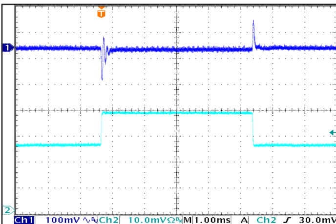
Figure 5: Output voltage response to step-change in load current (50%-75%-50% of I out (max); dI/dt = 0.1 A/μs). Load cap: 1 μF ceramic and 15 μF tantalum capacitors. Ch 1: V out , Ch 2: I out (0.2A/div).
