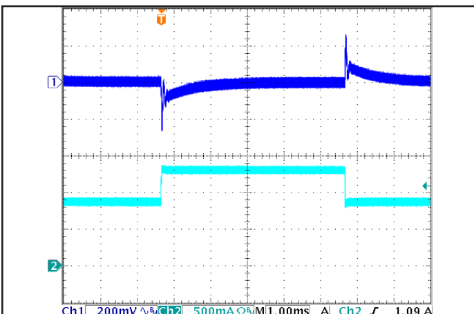
Figure 5: Output voltage response to step-change in load current (50%-75%-50% of I out (max); dI/dt = 0.1 A/μs). Load cap: 1 μF ceramic and 15 μF tantalum capacitors. Ch 1: V out , Ch 2: I out (0.5A/div).
