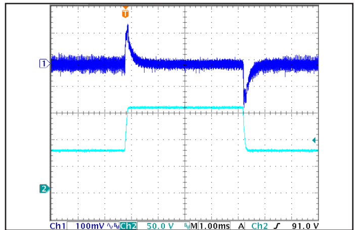
Figure 6: Output voltage response to step-change in input voltage (715V/ms), at Max. load current. Load cap: 15µF tantalum cap and 1µF ceramic cap. Ch 1: Vout, Ch 2: Vin.
