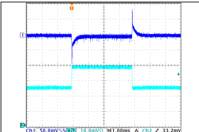
Figure 5: Output voltage response to step-change in load current (50%-75%-50% of Iout(max); dI/dt = 0.1A/µs. Load cap: 15µF tantalum cap and 1µF ceramic cap. Ch 1: Vout, Ch 2: Iout(1.0A/div).
