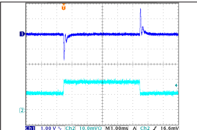
Figure 5: Output voltage response to step-change in load current (50%-75%-50% of I_{out(max)} ; dI/dt = 0.2 A/\mu s ). Load cap: 1 \mu F ceramic capacitor. Ch 1: V_{out} , Ch 2: I_{out} .
