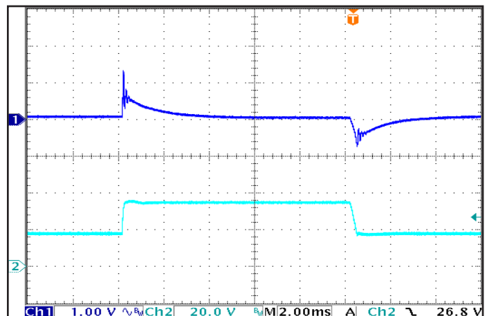
Figure 6: Output voltage response to step-change in input voltage (250 V/ms, V nom -V max -V nom ). Load cap: 1 μF ceramic capacitor. Ch 1: V out , Ch 2: V in .
