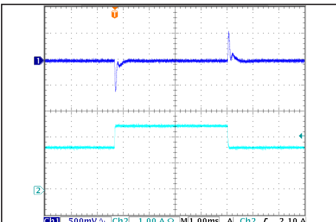
Figure 5: Output voltage response to step-change in load current (50%-75%-50% of Iout(max); dI/dt = 0.1A/\mu s ). Load cap: 1 \mu F ceramic and 15 \mu F tantalum capacitors. Ch 1: Vout, Ch 2: Iout (1A/div).
