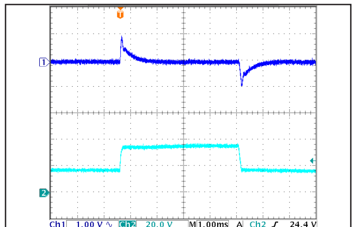
Figure 6: Output voltage response to step-change in input voltage (250 V/ms, V_{nom}-V_{max}-V_{nom} ). Load cap: 1 \mu F ceramic and 15 \mu F tantalum capacitors. Ch 1: Vout, Ch 2: Vin.
