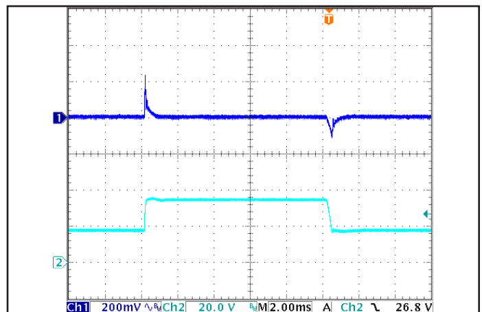
Figure 6: Output voltage response to step-change in input voltage (250 V/ms, V nom -V max -V nom ). Load cap: 1 μF ceramic and 15 μF tantalum capacitors. Ch 1: V out , Ch 2: V in .
