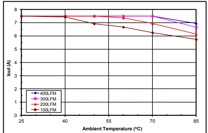
Figure 4: Encased Converter (0.7" heatsink) max. output current derating vs. ambient air temperature for airflow rates of 100 LFM through 400 LFM. Air flows across the converter from input to output (nominal input voltage).
