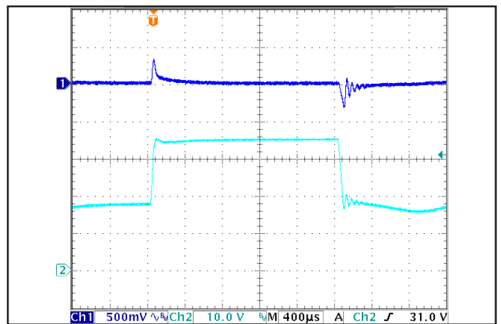
Figure 6: Output voltage response to step-change in input voltage (1V/μs). Load cap: 1 ¼F ceramic and 15 ¼F tantalum capacitors. Ch 1: V out , Ch 2: V in .
