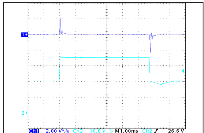
Figure 6: Output voltage response to step-change in input voltage (1V/μs). Load cap: 1 ¼F ceramic and 15 ¼F tantalum capacitors. Ch 1: Vout, Ch 2: Vin.
