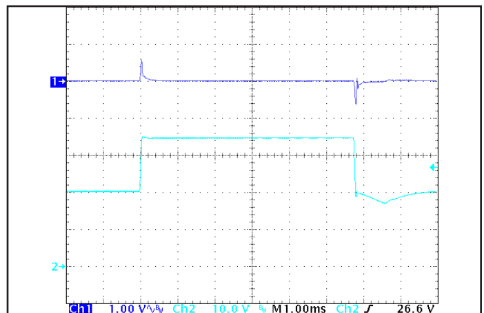
Figure 6: Output voltage response to step-change in input voltage (1V/μs). Load cap: 1 1/4F ceramic and 15 1/4F tantalum capacitors. Ch 1: Vout, Ch 2: Vin.
