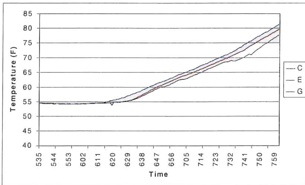
Figure 4. Variation of Temperature during Morning Session
