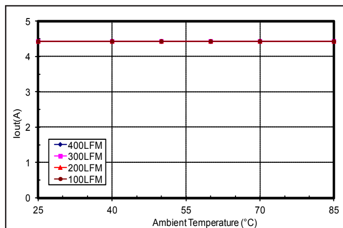
Figure 4: Encased Converter (0.7" heatsink) max. output current derating vs. ambient air temperature for airflow rates of 100 LFM through 400 LFM. Airflows across the converter from input to output (nominal input voltage).
