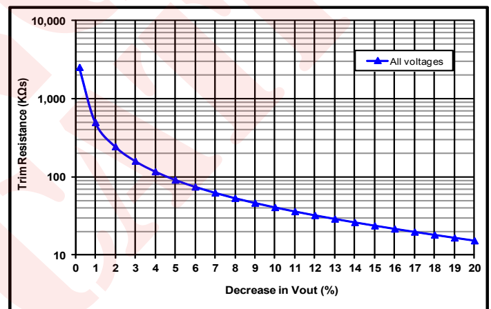
Common Figure 4: Trim graph for trim down.
