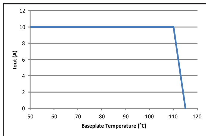
Figure 4: Maximum load current vs. baseplate temperature when conductively cooled. Note: The system design must provide a suitable thermal path that maintains the baseplate temperature below 110 °C.
