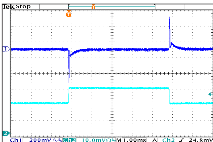
Figure 5: Output voltage response to step-change in load current (50%-75%-50% of I_{out(max)} ; dI/dt = 0.1 A/\mu s ). Load cap: 1 \frac{1}{4}F ceramic and 15 \frac{1}{4}F tantalum capacitors. Ch 1: V_{out} , Ch 2: I_{out} (2A/div)
