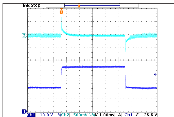
Figure 6: Output voltage response to step-change in input voltage (1000 V/ms). Load cap: 1 \mu F ceramic capacitor. Ch 1: V_{in} , Ch 2: V_{out} .
