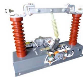
Disconnecter Inverters
