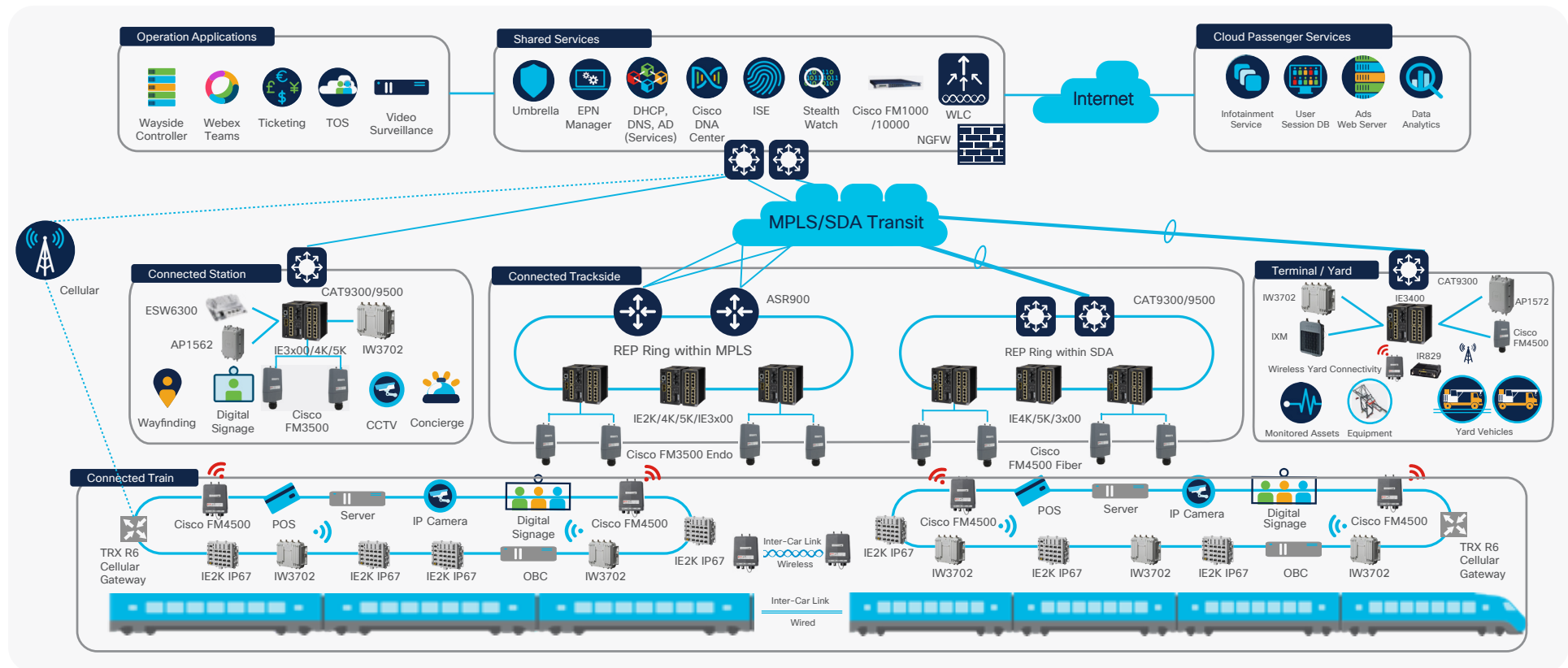
Figure 1. Connected Rail reference architecture
